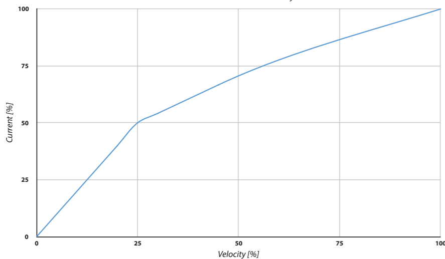
4–20 mA current versus velocity
