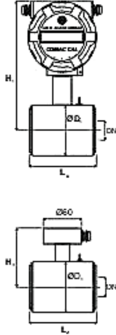
WAFER
